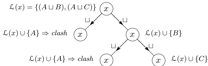
Figure 6: Syntactic branching search
