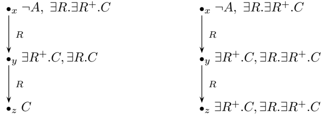
Figure 2: Dynamic blocking fails in the presence of transitive closure.
