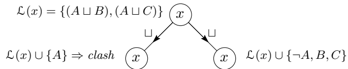
Figure 7: Semantic branching search
