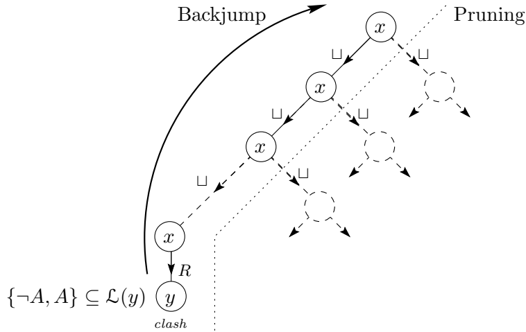
Figure 9: Pruning the search using backjumping
