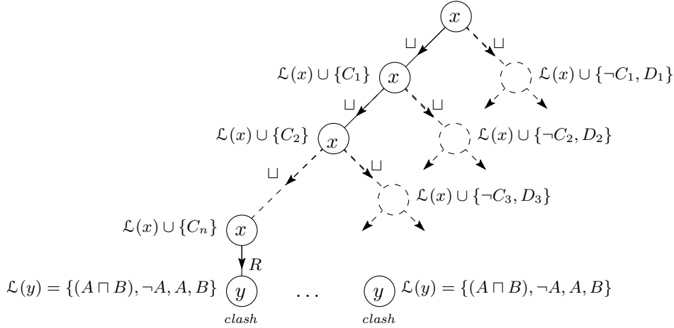
Figure 8: Thrashing in backtracking search
